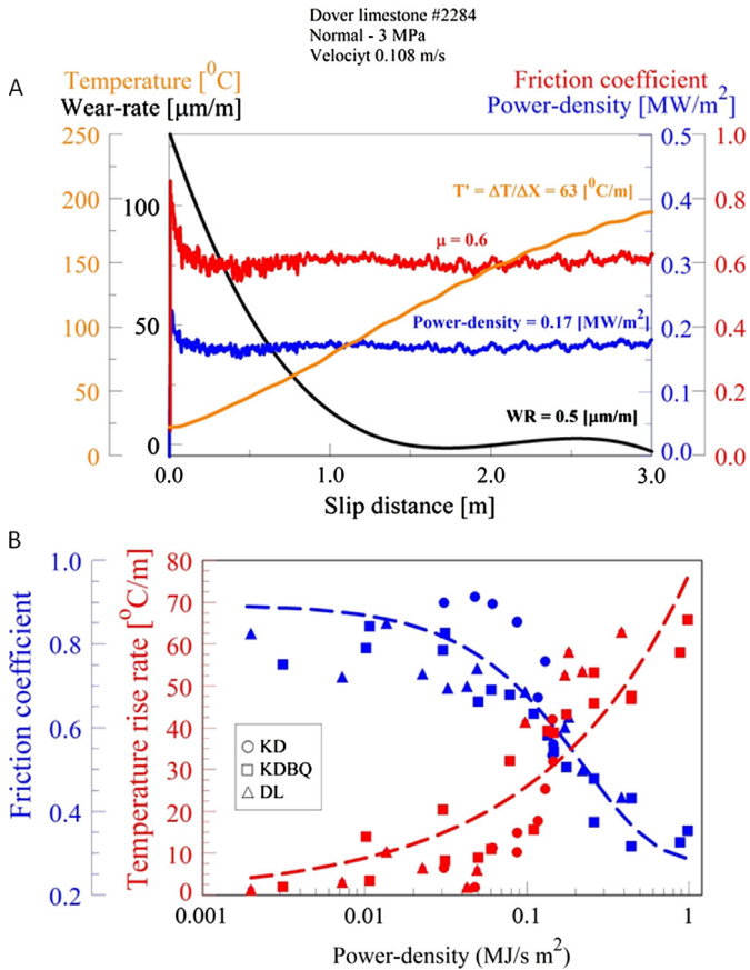
Fig. 10. A. Experimental evolution during steady-state experiment with Dover limestone; note that after ~1 m of slip, the power-density, friction coefficient, wear-rate and temperature slope all have quasi-constant values. B. Experimental relations between power-density PD and both friction coefficient, \mu (blue), and temperature-rise-rate, T' (red). Results of 12 runs with dis-functioning thermocouples were excluded from this plot. Also plotted best fit curves (dashed lines of Eqs. (4) and (5) in the text). Note the inverse dependency of m and T' on PD.
